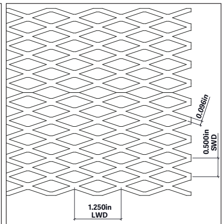
Steel Expanded Flat (1/2" - #16)
