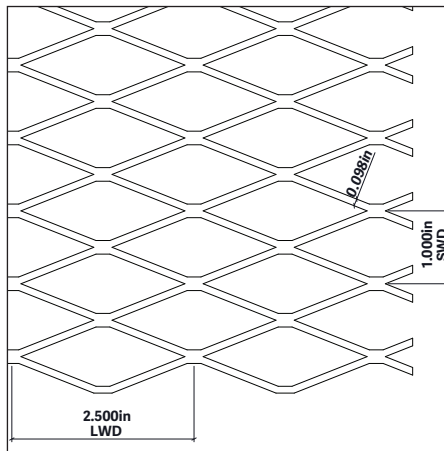
Steel Expanded Flat (1" - #16)
