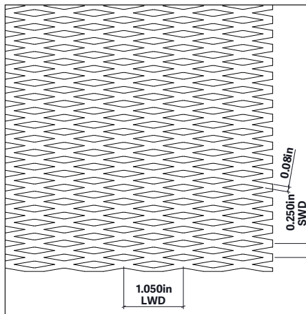
Steel Expanded Flat (1/4" - #18)
