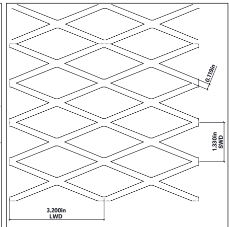
Steel Expanded Flat (1-1/2" - #16)
